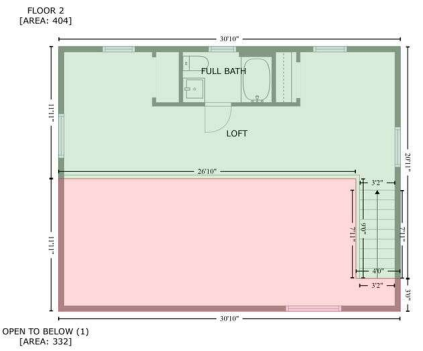
FLOOR 2 [AREA: 404]
