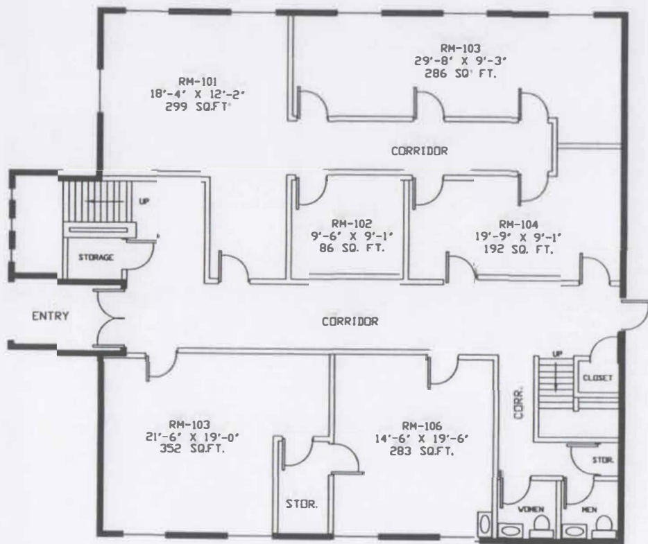
1ST FLOOR 2475 SQ. FT
