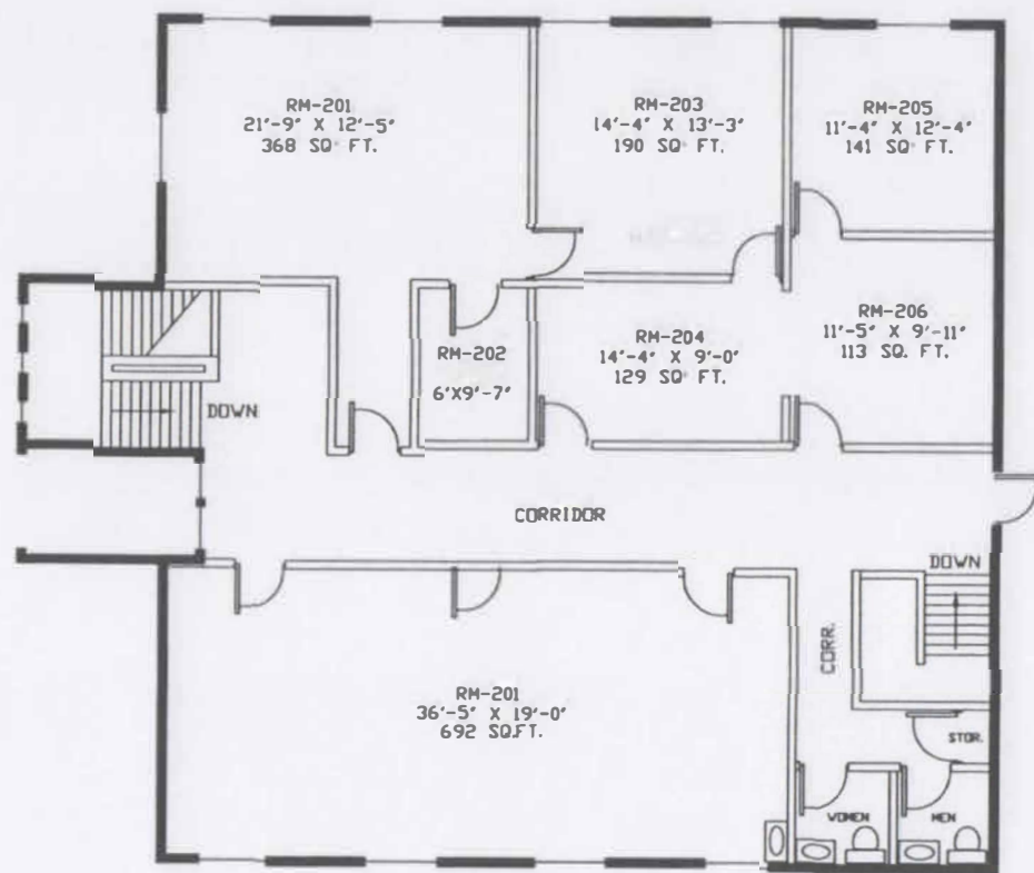
2ND FLOOR 2475 SQ. FT.
